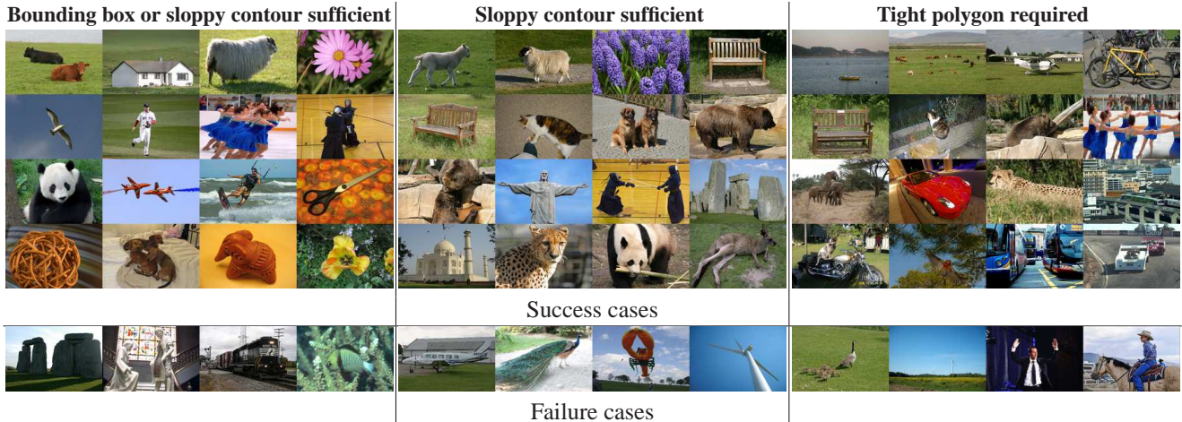
Figure 4: Example success (top) and failure cases (bottom) for our method, per annotation modality. Best viewed on pdf.
