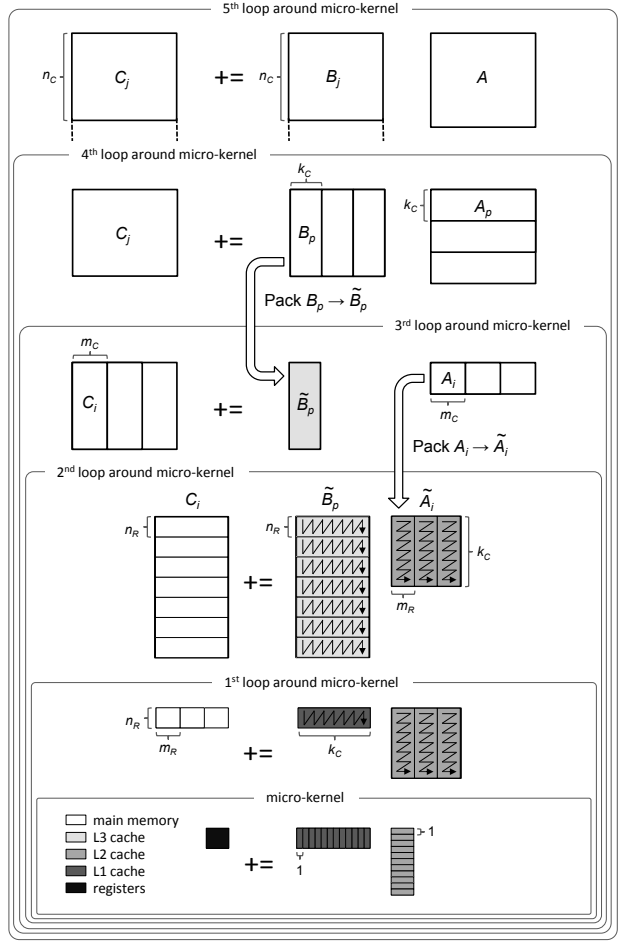
Figure 1: Left: An illustration of the algorithm for computing high-performance matrix multiplication, taken from [9], which expresses computation in terms of a so-called “block-panel” subproblem (macro-kernel). Right: An alternate algorithm that expresses the operation in terms of “panel-block” matrix multiplication.
