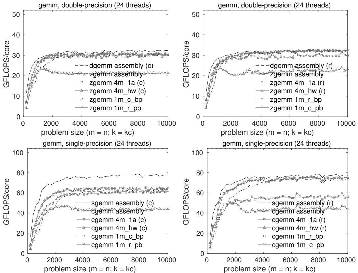
Figure 8: Multithreaded performance of various implementations of double-precision (top) and single-precision (bottom) complex GEMM on two Intel Xeon E5-2690 v3 “Haswell” processors, each with 12 cores. All data points reflect the use of 24 threads. The left and right graphs contain an identical reference curve for assembly-coded complex GEMM as well as results for three additional reference implementations (corresponding to the assembly-coded real GEMM, as well as 4M_1A and 4M_HW). These latter three implementations differ from left to right graphs in the preference of their underlying micro-kernel, indicated by a “(c)” or “(r)” (for column- or row-prefering). The left and right graphs also differ in which 1M implementations they report, with the left graphs reporting 1M_C_BP and 1M_R_PB (which employ column-prefering micro-kernels) and the right graphs reporting 1M_R_BP and 1M_C_PB (which employ row-prefering micro-kernels). The theoretical peak performance coincides with the top of each graph.
