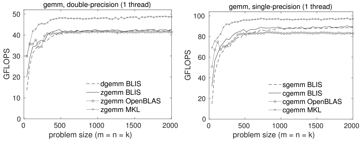
Figure 5: Single-threaded performance of various conventional (i.e., assembly-coded) implementations of double-precision (left) and single-precision (right) complex GEMM on a single core of an Intel Xeon E5-2690 v3 “Haswell” processor. The theoretical peak performance coincides with the top of each graph.
