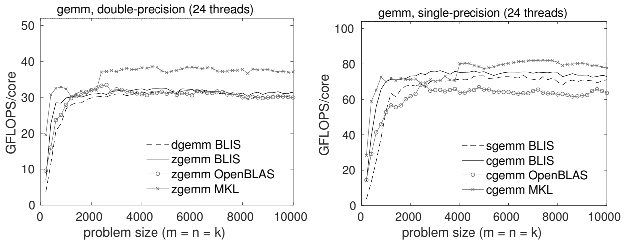
Figure 6: Multithreaded performance of various conventional (i.e., assembly-coded) implementations of double-precision (left) and single-precision (right) complex GEMM on 24 cores of an Intel Xeon E5-2690 v3 “Haswell” processor. The theoretical peak performance coincides with the top of each graph.
