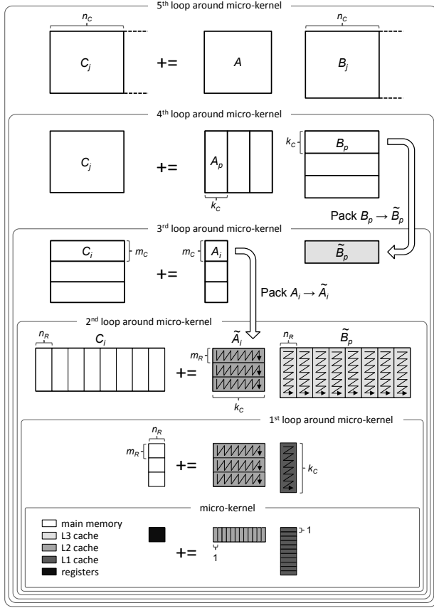
Block-panel-based GEMM
