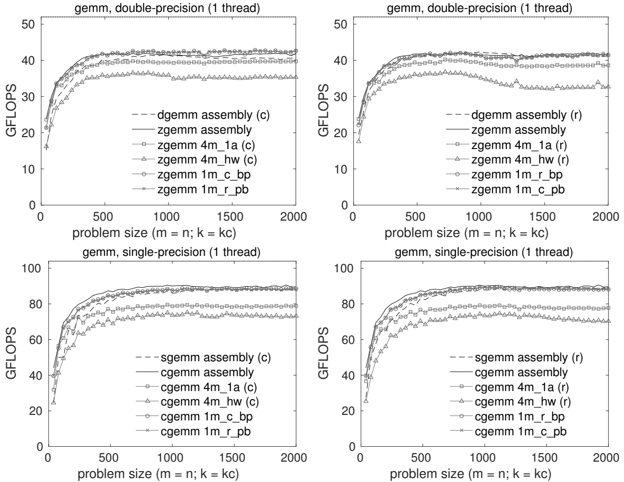
Figure 7: Single-threaded performance of various implementations of double-precision (top) and single-precision (bottom) complex GEMM on a single core of an Intel Xeon E5-2690 v3 “Haswell” processor. The left and right graphs contain an identical reference curve for assembly-coded complex GEMM as well as results for three additional reference implementations (corresponding to the assembly-coded real GEMM, as well as 4M_1A and 4M_HW). These latter three implementations differ from left to right graphs in the preference of their underlying micro-kernel, indicated by a “(c)” or “(r)” (for column- or row-prefering). The left and right graphs also differ in which 1M implementations they report, with the left graphs reporting 1M_C_BP and 1M_R_PB (which employ column-prefering micro-kernels) and the right graphs reporting 1M_R_BP and 1M_C_PB (which employ row-prefering micro-kernels). The theoretical peak performance coincides with the top of each graph.
