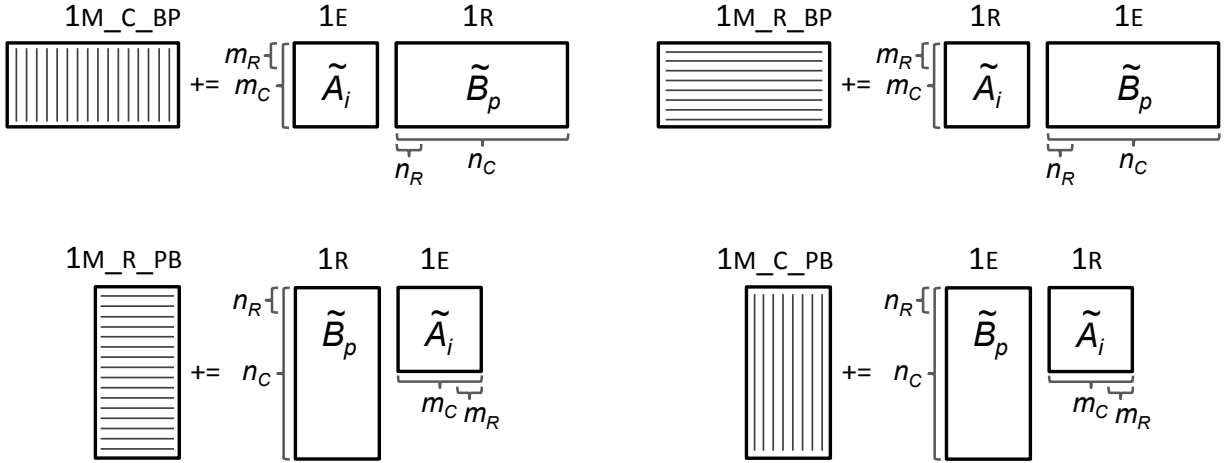
Figure 4: Illustrations that depict key details of the four 1M algorithms at the level of the macro-kernel, including the 1E/1R packing formats of \tilde{A}_i and \tilde{B}_p , whether each packed matrix is a left- or right-hand operand to the matrix product, and the corresponding relationship between the m and n dimensions and the cache and register blocksizes m_C , m_R , n_C , and n_R . In each diagram, the storage of the output matrix prescribed by the 1M_C/1M_R variant is shown as vertical (column-stored) or horizontal (row-stored) lines. The algorithms represented by the diagrams on the left will exhibit similar performance properties when the matrices are large. A similar relationship holds between the pair of algorithms on the right.
