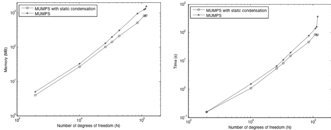
Figure 1: Memory and time savings from Static Condensation before the application of the Mumps solver.
