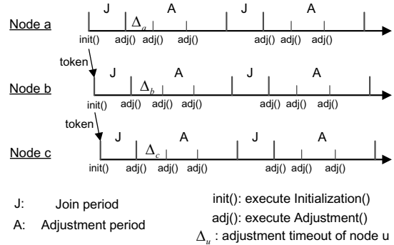
Fig. 4. Main structure of VPoD
