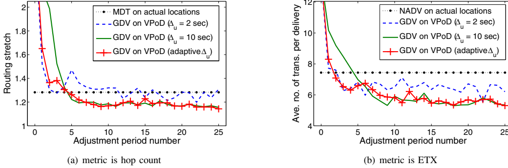
Fig. 8. Routing performance for different timeout values
