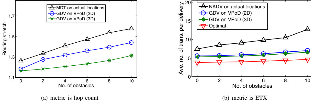
Fig. 13. Routing performance vs. number of obstacles
