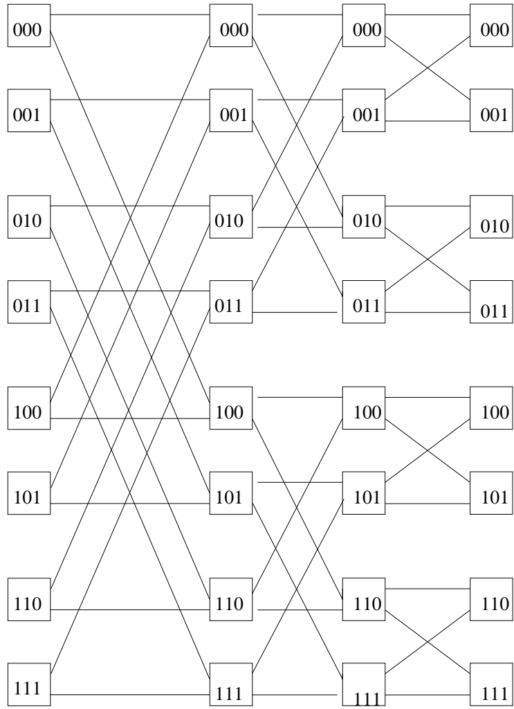
Figure 1: Butterfly Network, N = 8
