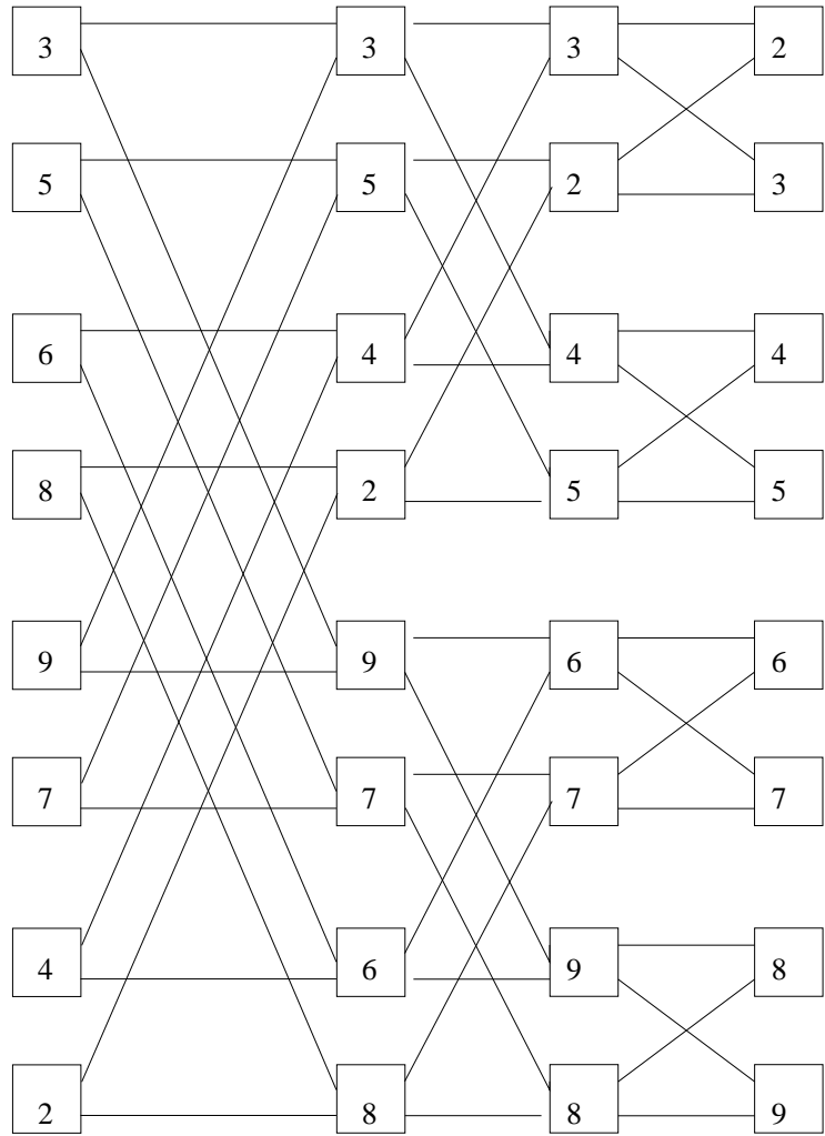
Figure 2: Merging sorted lists on a Butterfly Network, N = 8
