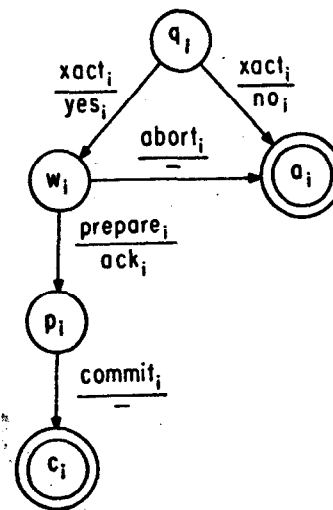
Figure 7. A (three phase) nonblocking central site commit protocol.
