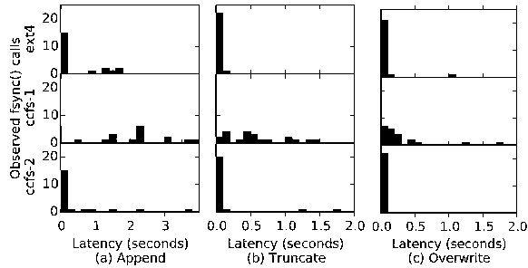
Figure 4: Repeated f_{\text{sync}} Experiments Histogram of user-observed foreground latencies in our multi- f_{\text{sync}} experiments. Each experiment is run for two minutes on a HDD.
