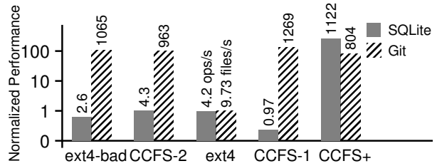
Figure 6: Case Study: Multiple Application Performance. Performance of Git and SQLite-rollback run simultaneously under different configurations on HDD, normalized to performance under ext4 configuration. Ext4-bad configuration runs the applications on ext4 with consistency sacrificed in Git. CCFS-2 uses separate streams for each application on ccfs. Ext4 uses ext4 with consistent Git. CCFS-1 runs both applications in the same stream on ccfs. CCFS+ runs applications in separate streams without unnecessary fsync . Workload: Git adds and commits a repository 25 times the size of Linux; SQLite repeatedly inserts 120-byte rows until Git completes.
