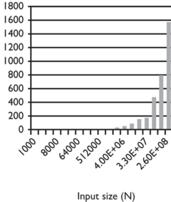
Figure 13.4 Runtimes for third version of range algorithm
