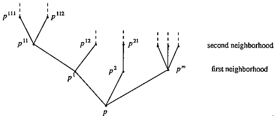
Figure 1: Singularity Tree
