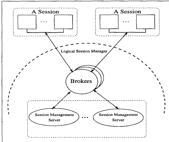
FIGURE 2: Brokered session management
