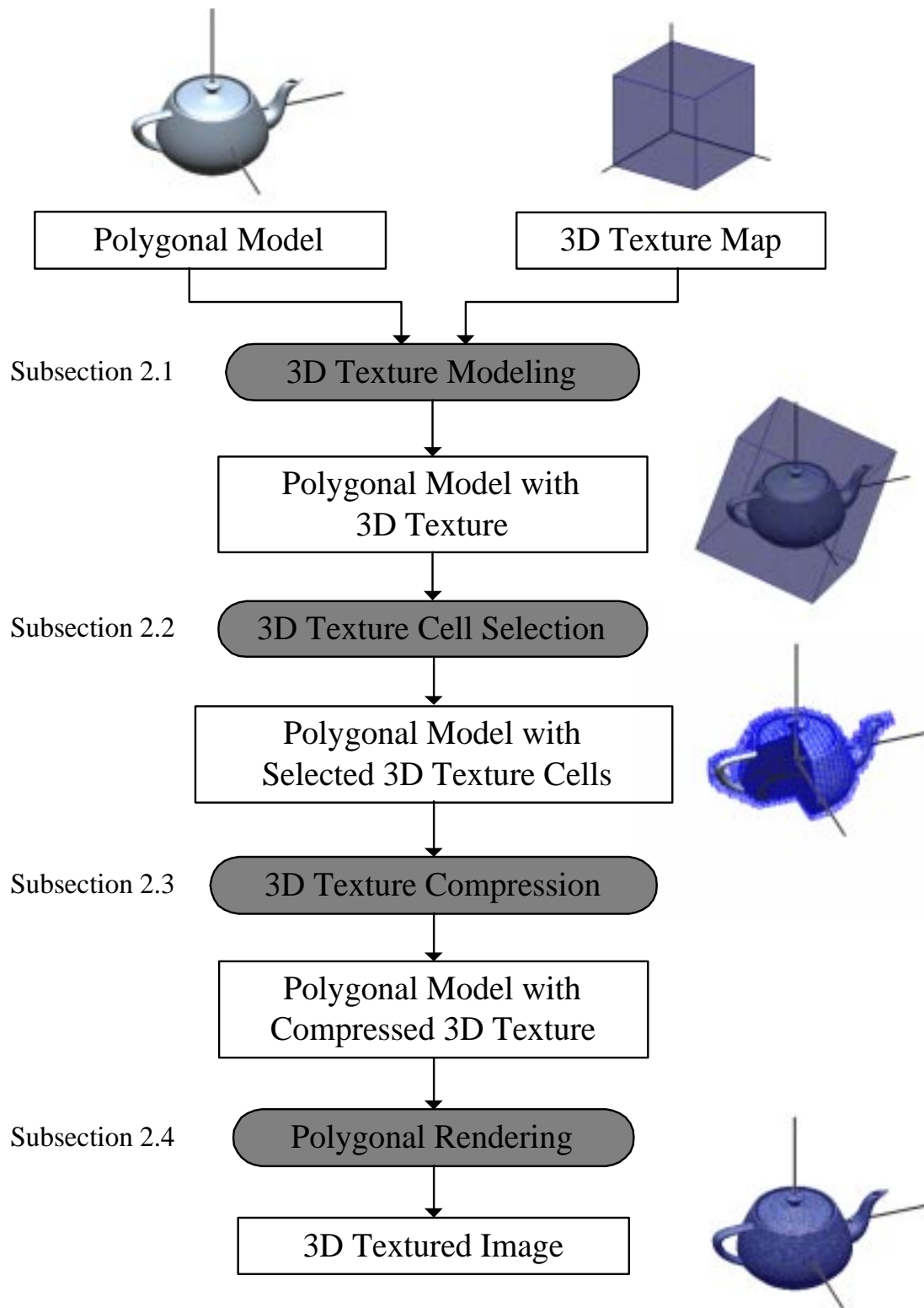
Figure 1: 3D Texture Mapping Pipeline
