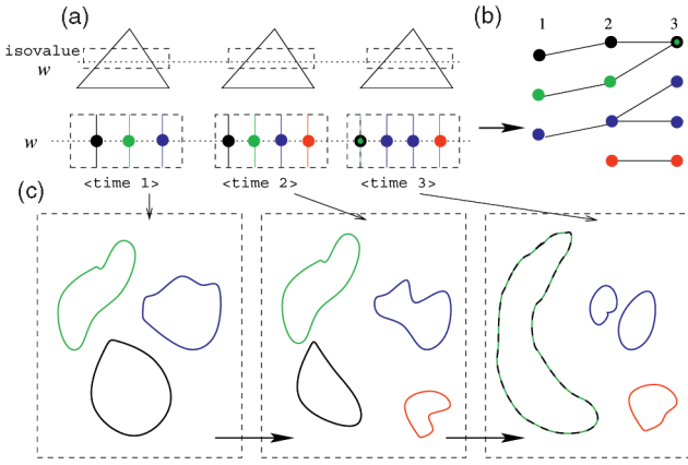
Fig. 1. Evolution of three isosurfaces. An intersection point on an edge of a contour tree represents a contour component. (a) By using precomputed correspondence information in time-dependent contour trees and (b) a graph representing the topology changes of time-varying isosurfaces is immediately constructed for any selected isovalue. (c) Seed sets generated from the contour trees are used for rapid extraction of the time-dependent surfaces of segmented contours. Note that colors represent correspondence among intersection points in contour trees, nodes of the graph, and contour components.
