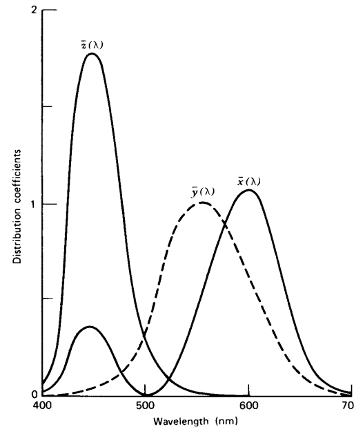
The XYZ color matching functions (Wasserman 3.8)
