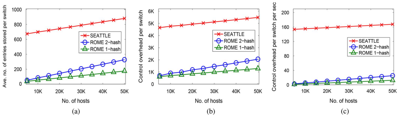
Fig. 6. Performance comparison by varying the number of hosts. (a) Storage cost. (b) Control overhead for initialization. (c) Control overhead in steady state.
