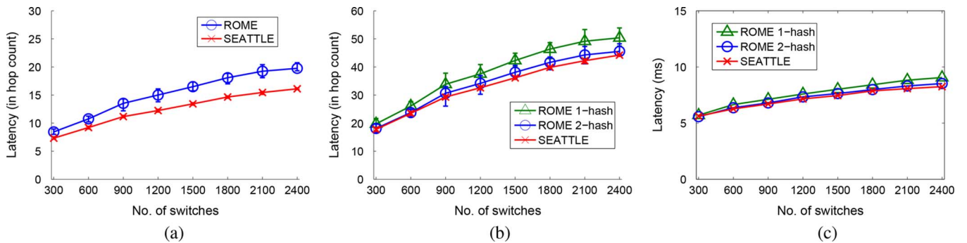
Fig. 8. Latency versus number of switches. (a) Packet to a discovered host. (b) First packet to an unknown host. (c) First packet to unknown host in hybrid nets.
