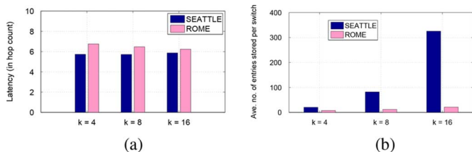
Fig. 9. Performance comparison for FatTrees. (a) Routing latency. (b) Storage cost.
