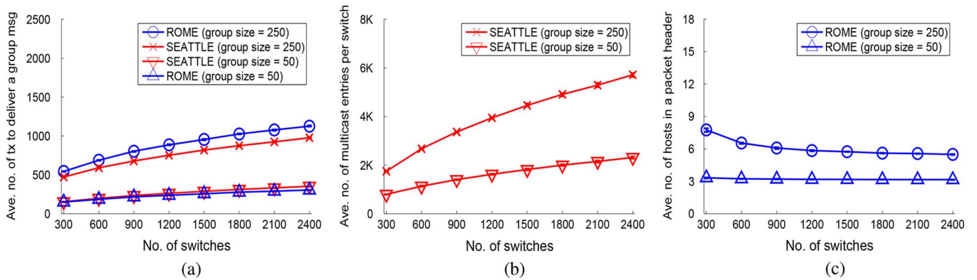
Fig. 11. Performance of multicast. (a) Average number of transmissions to deliver a group message. (b) Multicast storage cost per switch of SEATTLE. (c) Average number of destinations in the header of a ROME group message.
