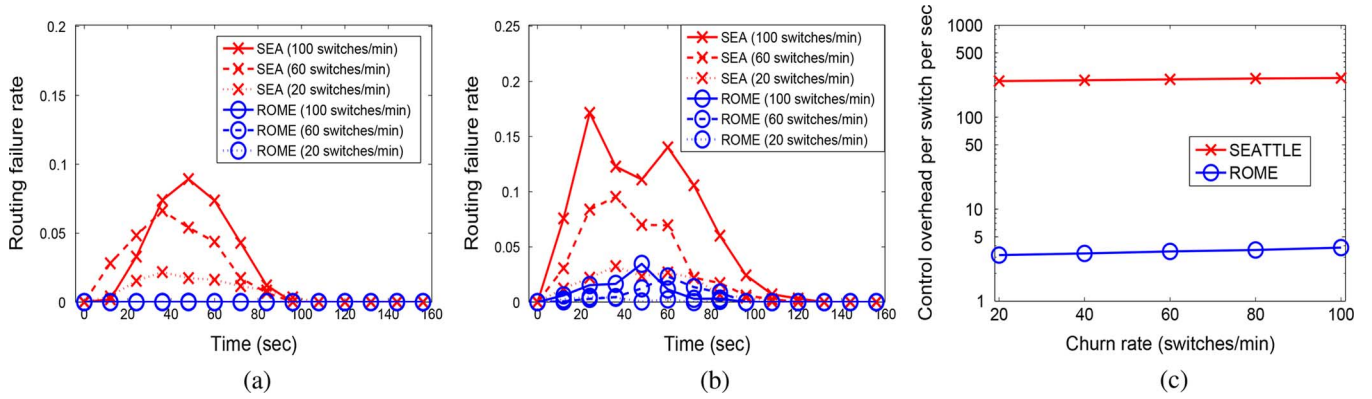
Fig. 10. Performance under network dynamics. (a) Routing failure rate to a discovered host. (b) Routing failure rate to an unknown host. (c) Control overhead.
