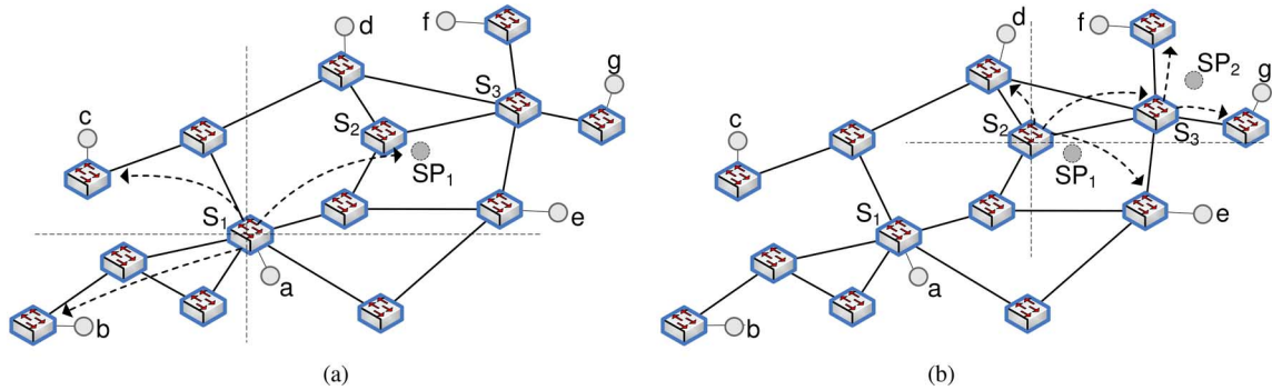
Fig. 1. Example of stateless multicast. (a) Split at S_1 . (b) Splits at S_2 and S_3 .
