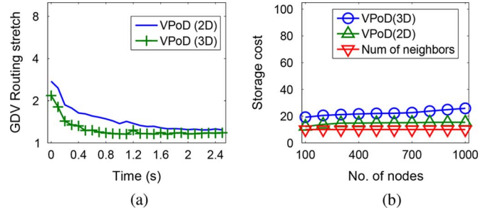
Fig. 5. Performance comparison for 2-D and 3-D virtual spaces. (a) Routing stretch convergence. (b) Storage cost.
