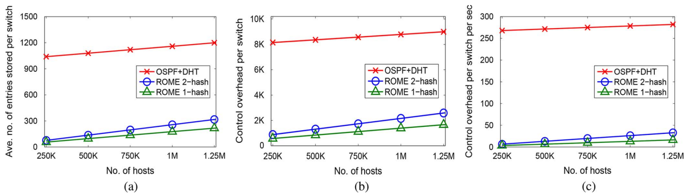
Fig. 13. Performance comparison for a very large hierarchical network (25 000 switches). (a) Storage cost. (b) Control overhead for initialization. (c) Control overhead in steady state.
