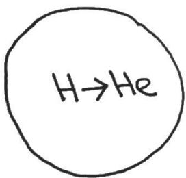
1. Main Sequence
