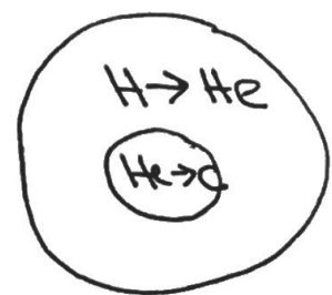
3. Horizontal Branch
