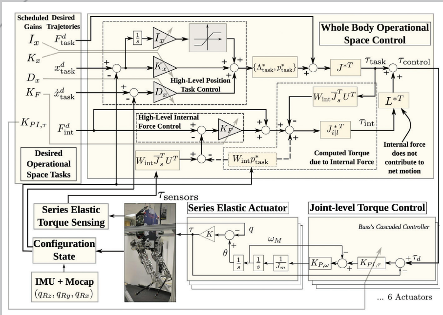
FIGURE 4 Schematic of the Whole-Body Operational Space Controller implemented in the Hume bipedal robot.
