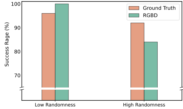
Fig. 7: IL Results in Simulation . Policy with RGBD input yields comparable performance to policy with ground truth chair positions as input.
