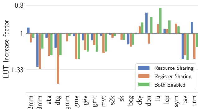
(a) LUT increase from resource sharing and register sharing.
