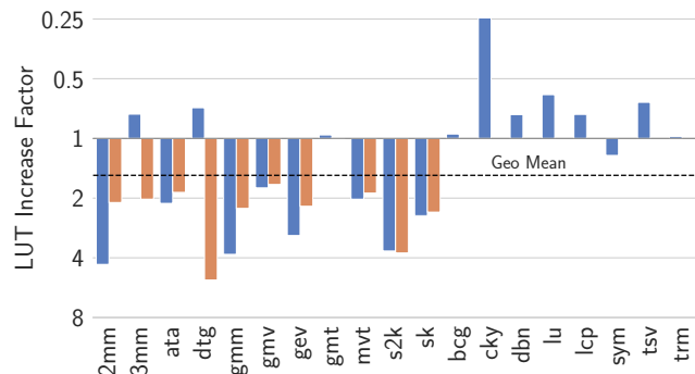
(b) LUT increase of Calyx designs over Vivado HLS. Designs below the y -axis are larger.
