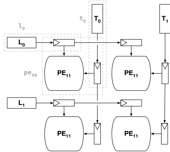
Figure 5: Architecture for a 2x2 by 2x2 matrix-multiply systolic array. Highlighted boxes show some of the groups used by the control.
