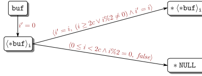
Fig. 1. The points-to graph at the end of function send_packets
