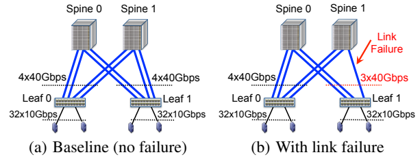
Figure 7: Topologies used in testbed experiments.
